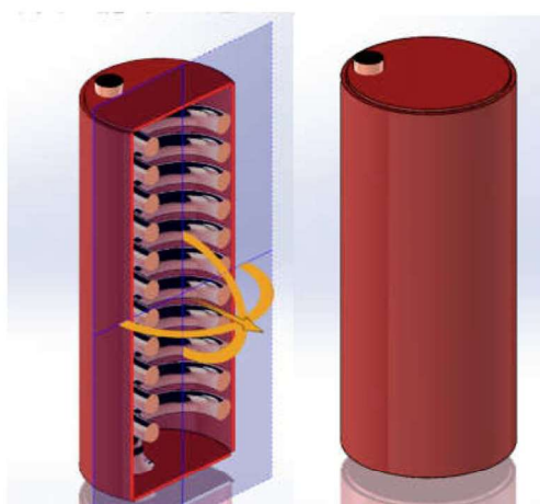
Figure 4. Evaporator Design
