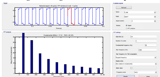
Fig.d. load current THD
