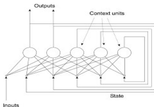
Fig.1.FULLY CONNECTED RNN
