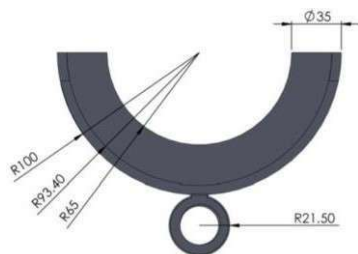
Figure 2: Top view of Nut-Gripper
