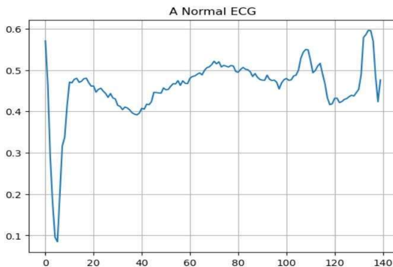
Figure 2. Normal ECG
