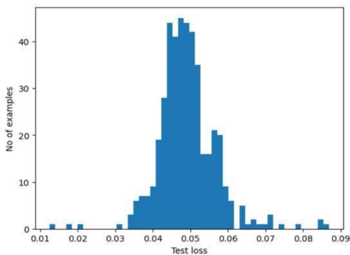
Figure 6. Testing loss
