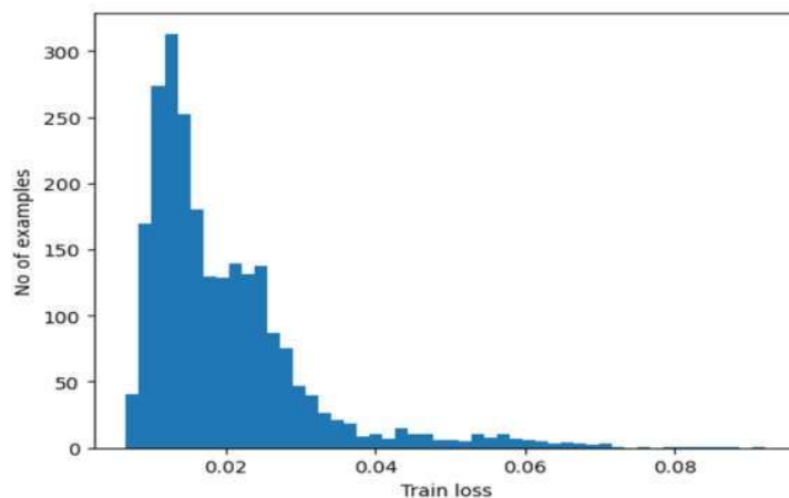
Figure 5. Training loss
