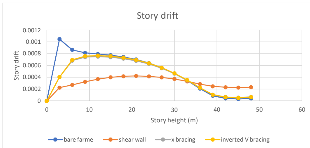
Comparative Graph Showing Drift in Y Direction
