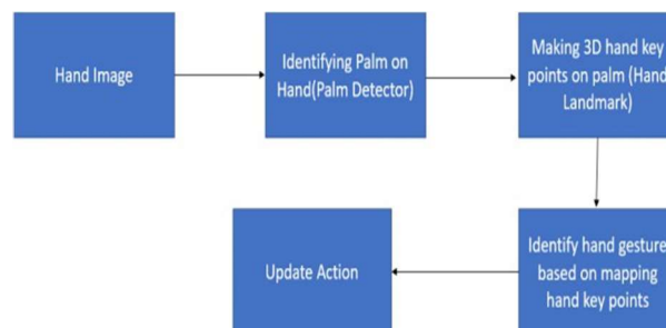
Figure 1: Architecture Diagram
